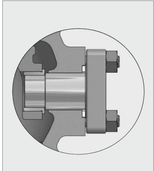
Figure 3: Post Bearing
